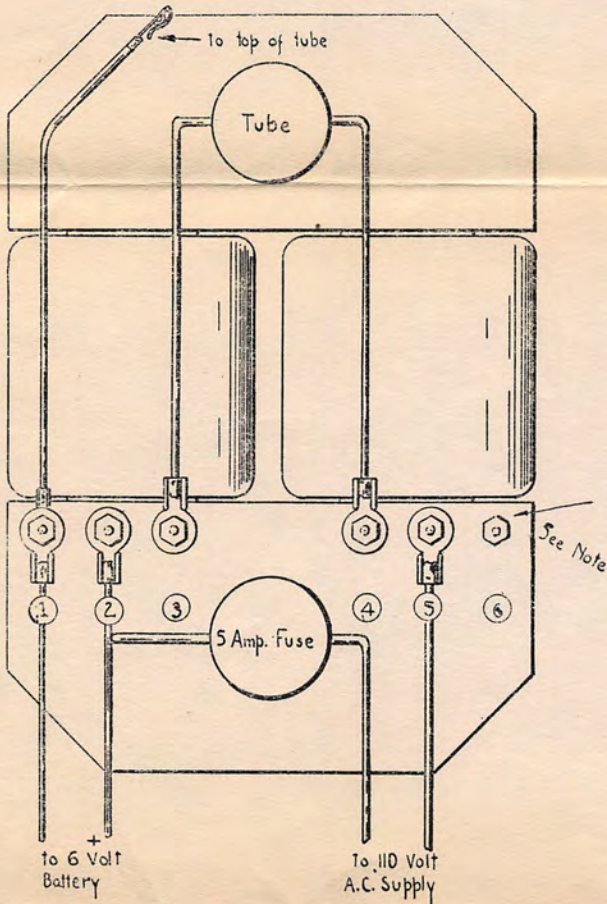
Diagram of Construction
