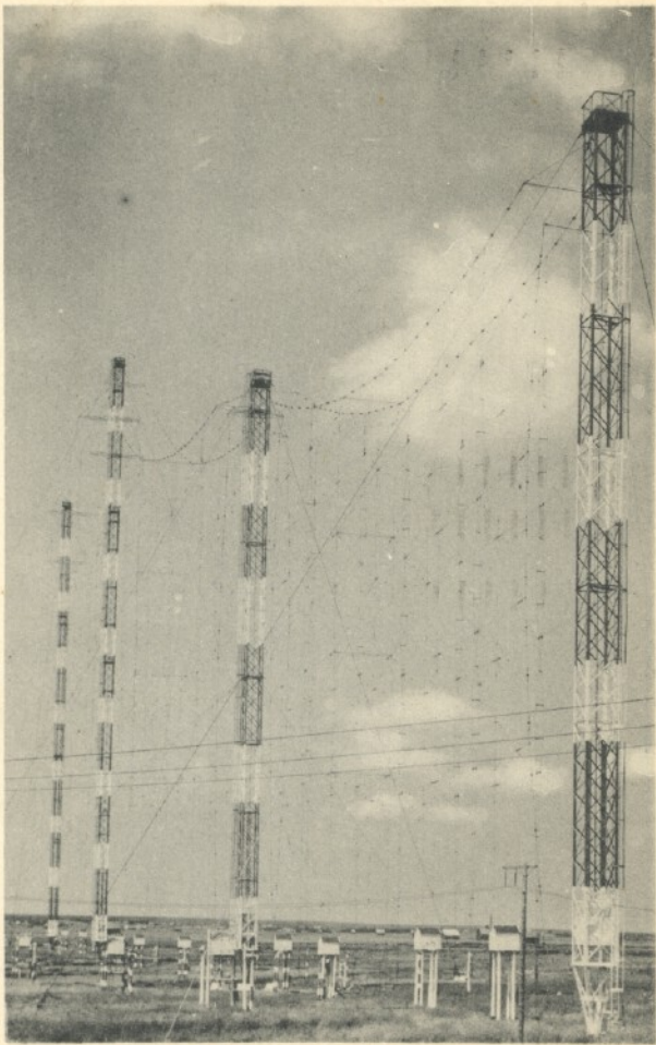
Shortwave Towers C.B.A., Sackville, N.B.
