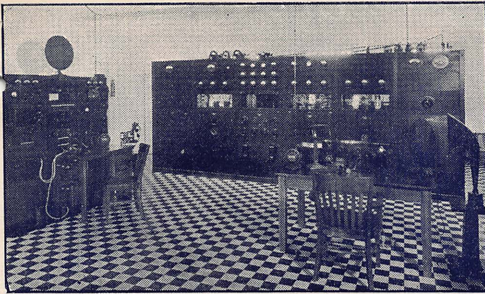
W P G 5000 Watt (Western Electric) Transmitter
