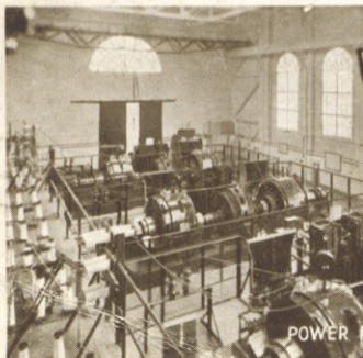
AMERICAN LONG WAVE TELEPHONY TRANSMITTER.
