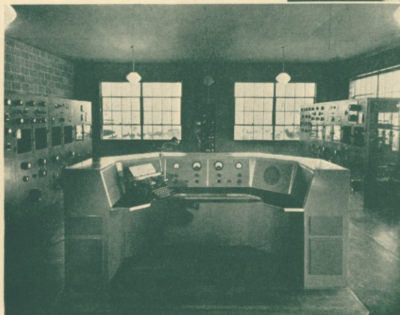
View of Transmitter Operating Room at Hatherly Beach, Mass. Twin Transmitters WRUL (left) and WRUW (right). Control desk in center governs both transmitters.
